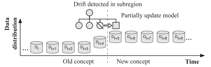
Fig. 15. A decision tree node is replaced with a new one as its performance deteriorates when a concept drift occurs in a subregion.
