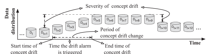
Fig. 11. An example of the occurrence time and the severity of concept drift. One incremental drift starts to change at t + 1 and ends at t + 5 . The other sudden drift occurs between t + 9 and t + 10 . The severity of these two concept drifts ( D_{t+1}-D_{t+5} and D_{t+9}-D_{t+10} ) is marked with brackets.
