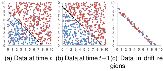
Fig. 12. An example of the drift regions of concept drift.
