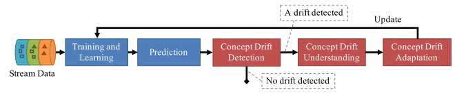
Fig. 2. Framework for handling concept drift in machine learning. Please note that some methods can do concept drift detection and concept drift understanding simultaneously.
