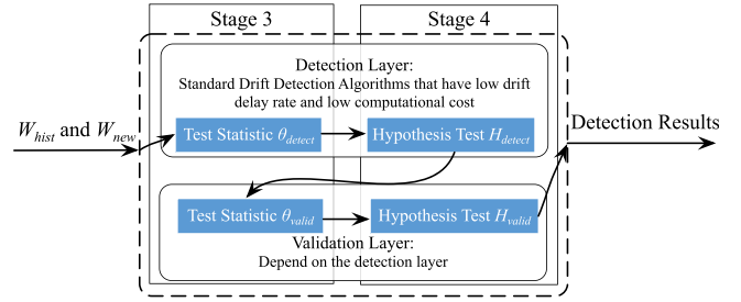
Fig. 10. Hierarchical multiple hypothesis test drift detection.
